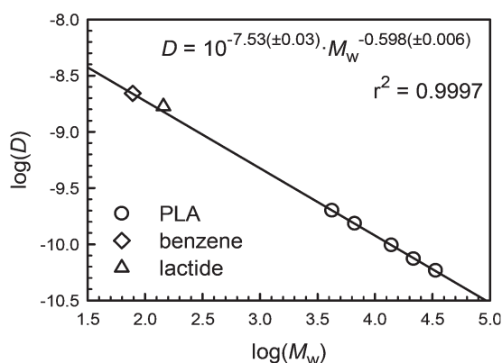
Fig. 1 Mass-averaged molar mass ( M_w ) vs. diffusion coefficient ( D ) log–log plot for PLA in benzene- \text{d}_6 .
